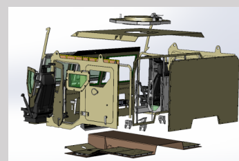
Cabin Kits SKD & CKD
