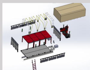
Fully customizable body systems/kits
